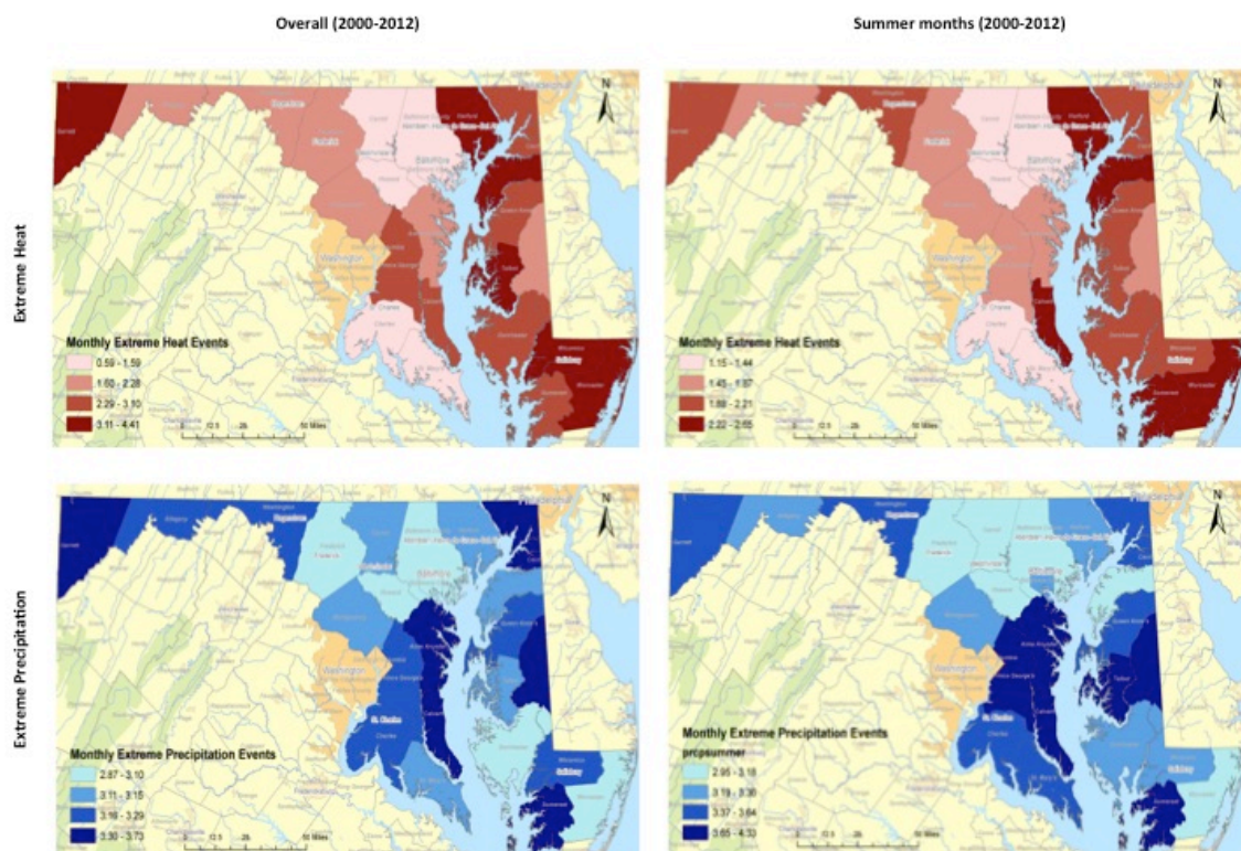
Figure 17. Number of extreme events by county, for overall years and during summer months (2000-2012).
