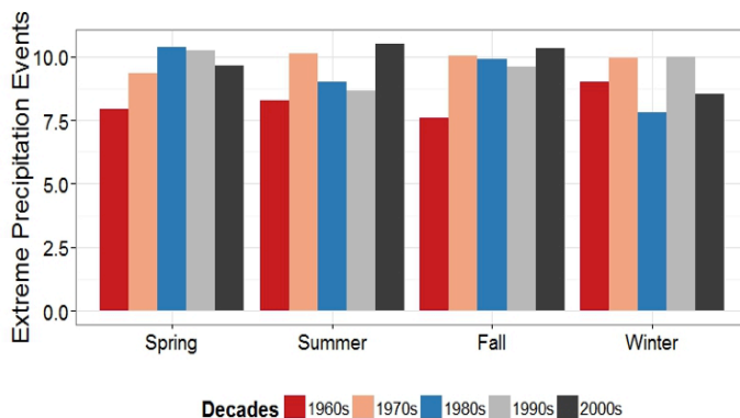
Figure 16. Temporal trend in extreme precipitation events (1960-2010), by season.
