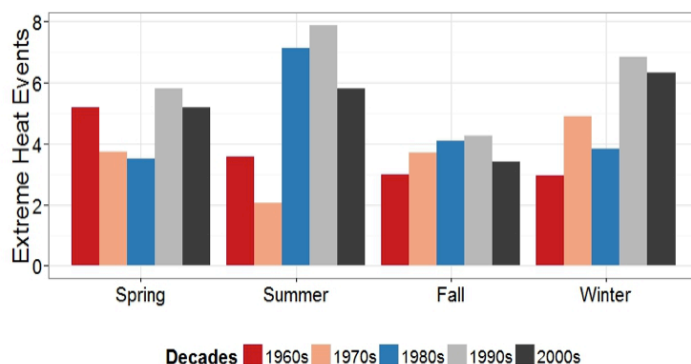
Figure 15. Temporal trend in extreme heat events (1960-2010), by season.
